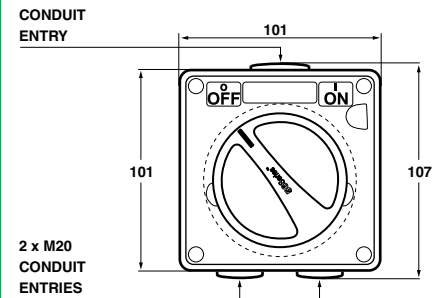
FRONT COMPLETE
