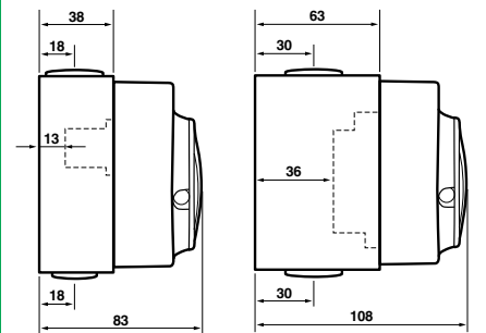
SIDE COMPLETE
