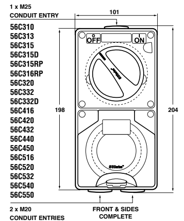
Dimensional Drawings
